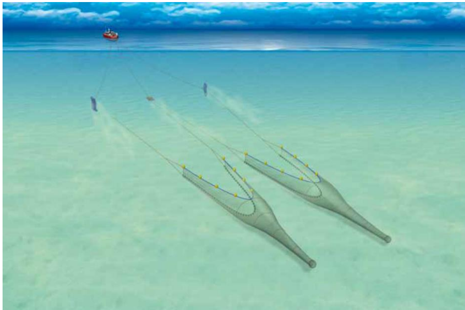
Figure A.4 Twin-rig Otter Trawl (Source: ©Seafish, 2015)
