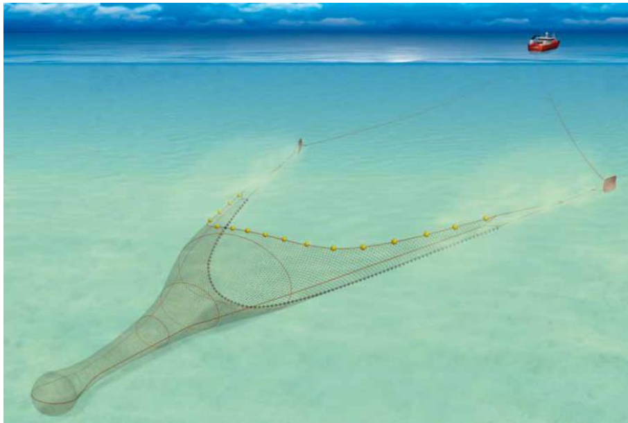
Figure A.3 Single-rig Otter Trawl (Source: ©Seafish, 2015)
