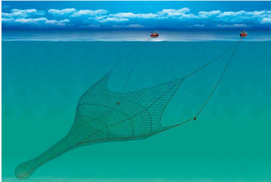
Figure A.5 Twin-rig Pelagic / Midwater trawl (Source: ©Seafish, 2015)
